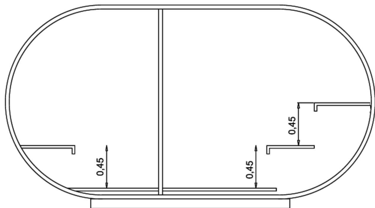
Oval sauna type 1
