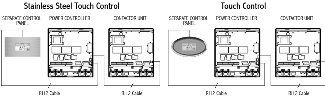
Fig.5 Installation of separate Control Panel and Power Controller with Contactor Unit
