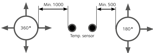
Forced ventilation diagram
