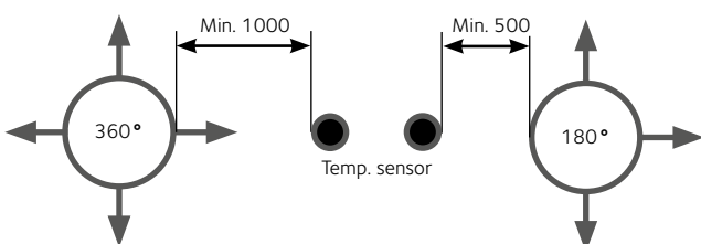
Forced ventilation diagram
